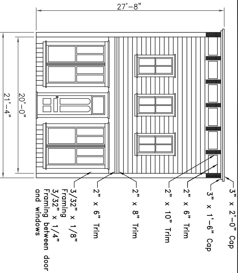
Front Elevation ( Plans & Elevations )
