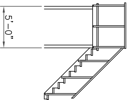
Rear Stairway ( Detail )
