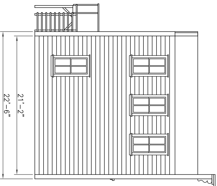
Side Elevation ( Plan & Elevation )
