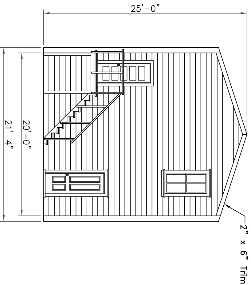
Rear Elevation ( Loading Platform )
